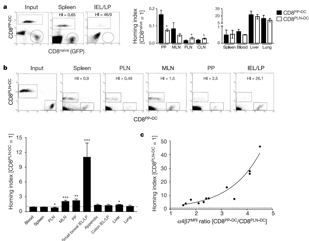
Figure 3 CD8 PP-DC home to the small intestine. P14 \times T-GFP cells were cultured for 6–7 days with gp33–41-pulsed DCs isolated from PLN or PP of the same donor pool. a , In one series, stimulated cells were labelled with TRITC and mixed with an equal number of T-GFP cells (containing ~35% GFP + naive T cells), and the homing index (HI, the ratio of [TRITC + cells] to [GFP + cells] in recipient blood or tissues divided by the input ratio) was determined in recipients' blood and tissues 4 h after adoptive transfer. FACS histograms (left) show a representative experiment comparing CD8 PP-DC and naive T-GFP cells (non-fluorescent input cells are non-T cells among donor splenocytes). Bar graphs (right) show mean \pm s.e.m. of three experiments (*, P < 0.05 compared with CD8 PP-DC ).
